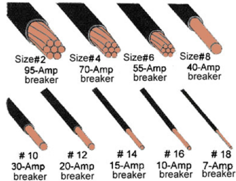
Circuit breaker and wire size chart
